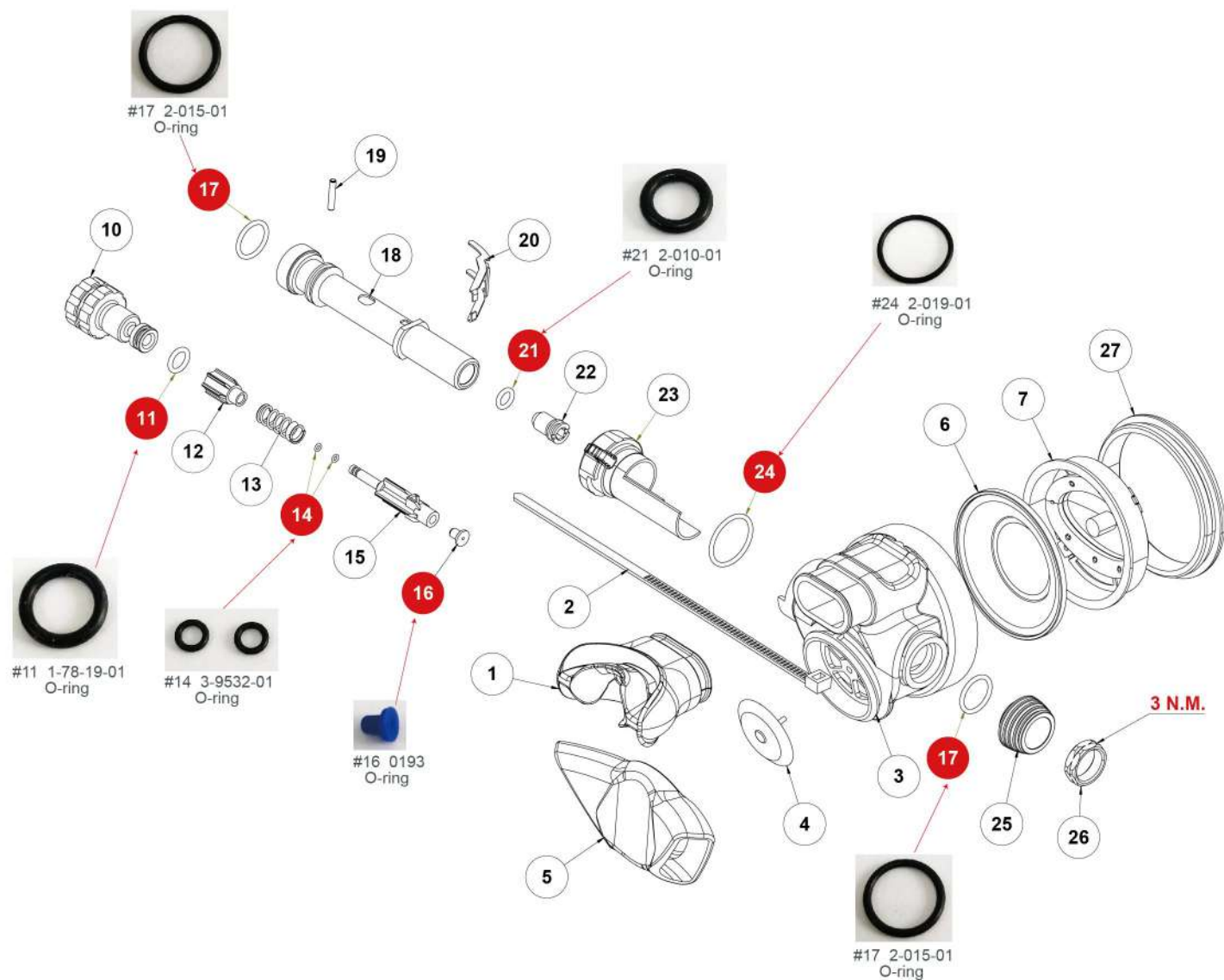
RO-19 2ND STAGE REG PART LIST
