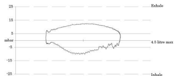
Pressure - Volume Diagrams at Mean Depth of : 50.4 msw (165.3 fsw)
