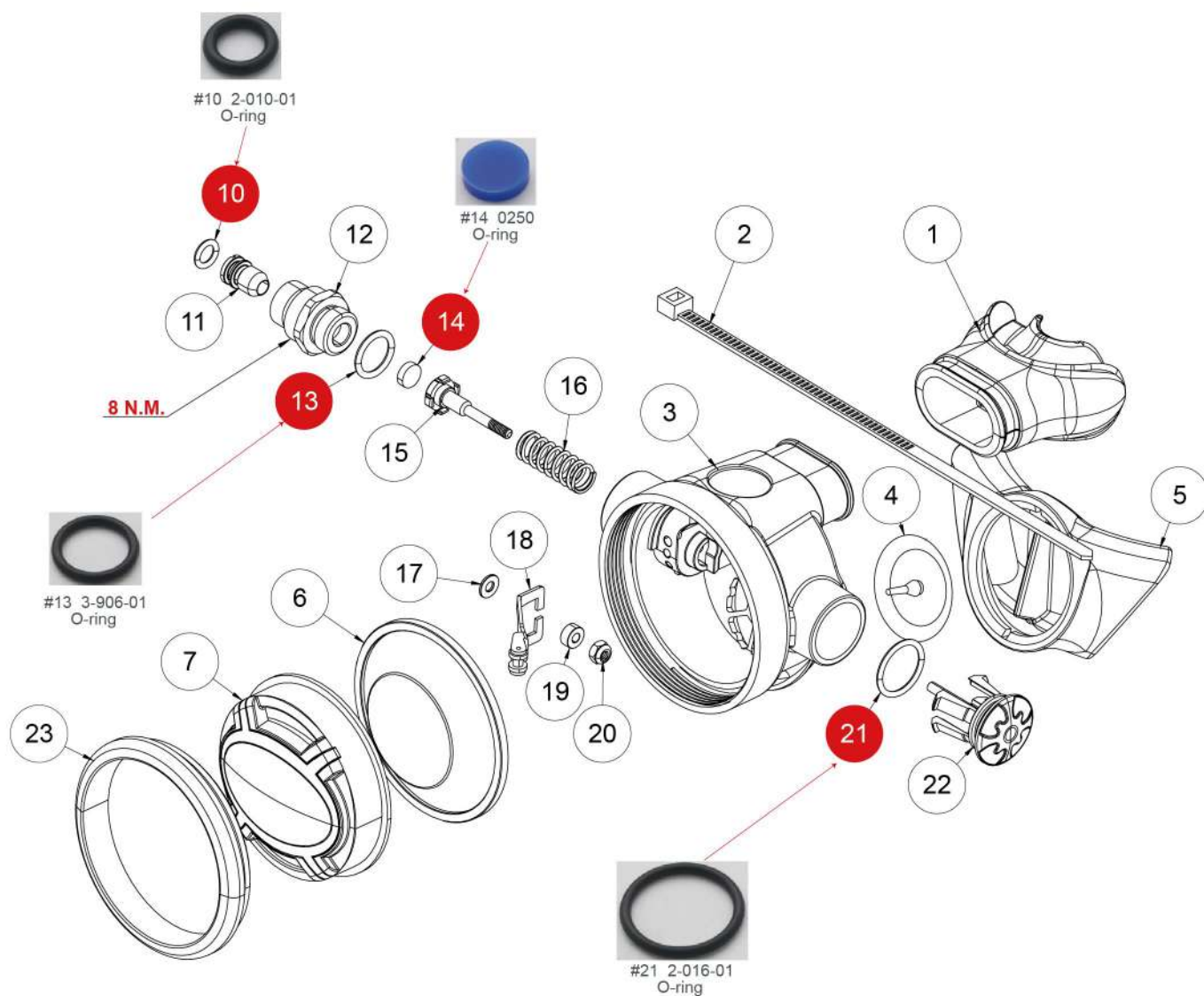
RO-20 2ND STAGE REG PART LIST
