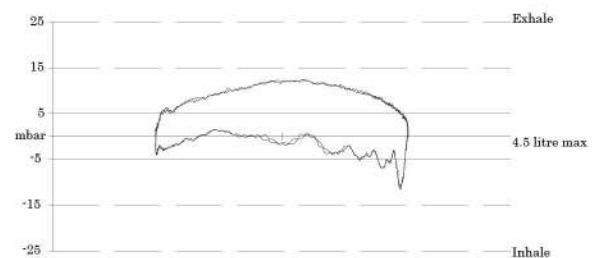
Pressure - Volume Diagrams at Mean Depth of : 50.3 msw (165.2 fsw)
