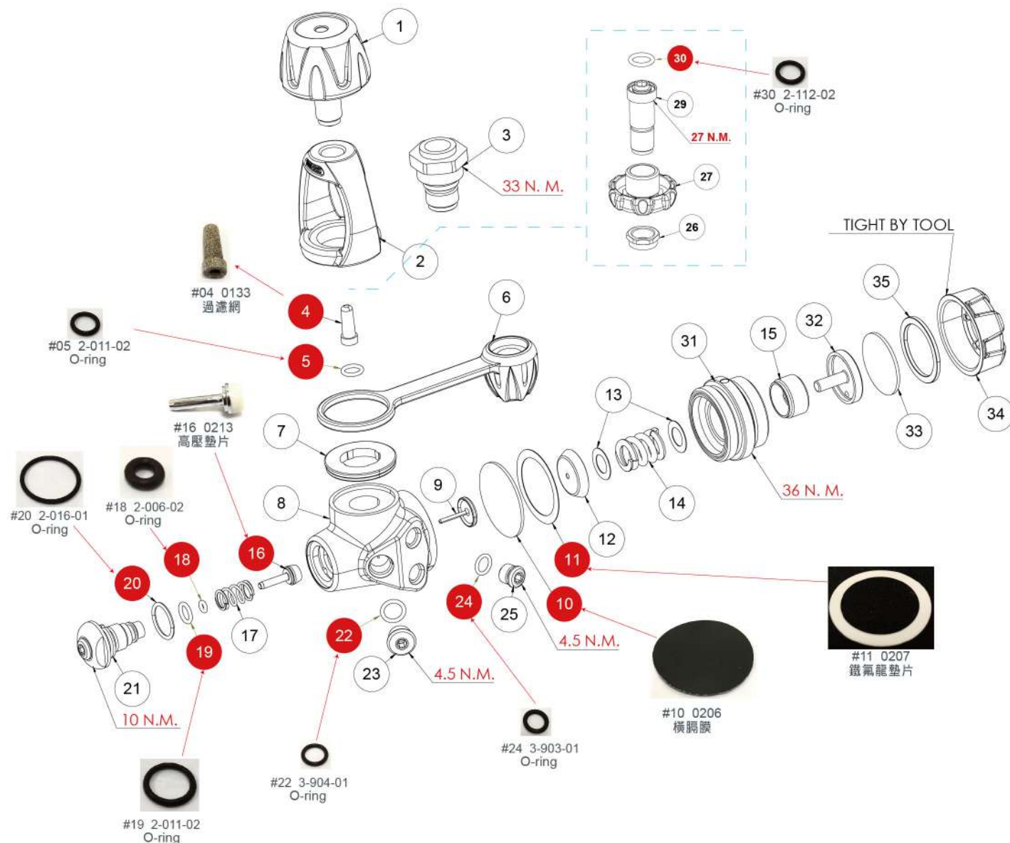
FS-850B DIAPHRAGM BALANCE REG PART LIST
