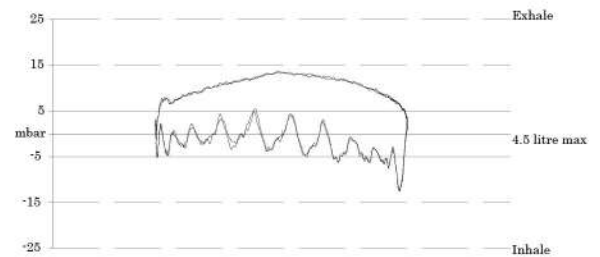
Pressure - Volume Diagrams at Mean Depth of : 51.8 msw (169.9 fsw)
