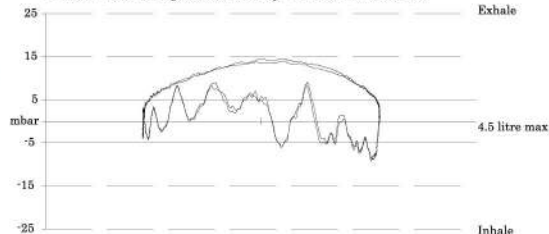
Pressure - Volume Diagrams at Mean Depth of : 51.5 msw (169.1 fsw)
