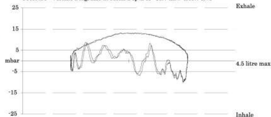
Pressure - Volume Diagrams at Mean Depth of : 51.7 msw (169.7 fsw)
